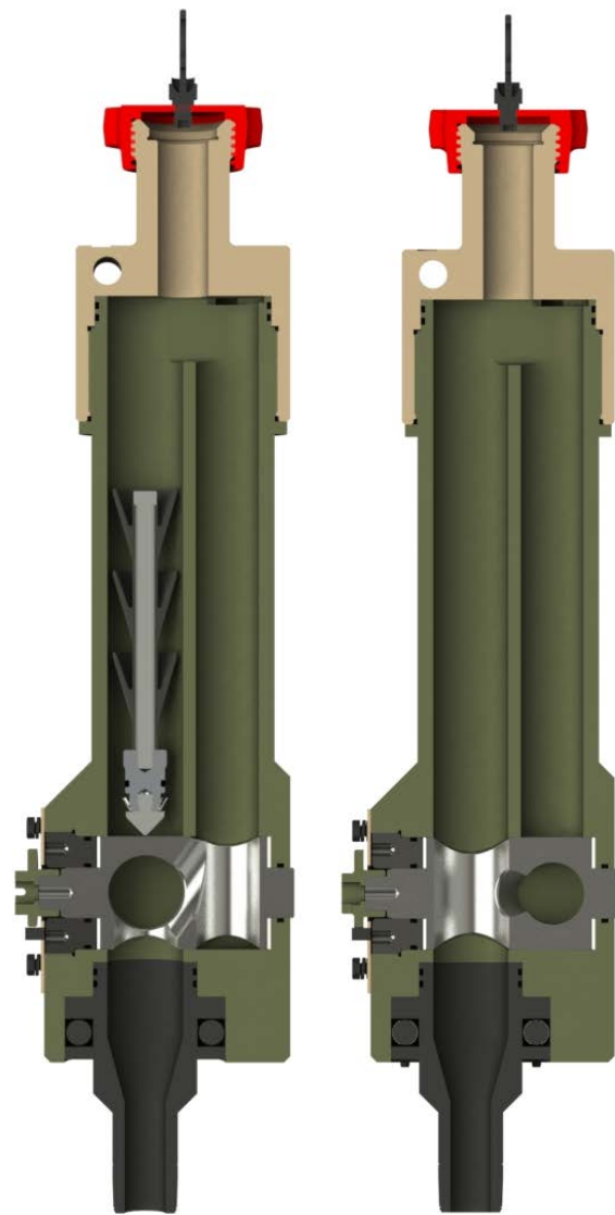
Preloaded Closed Chamber (left); Chamber Open, Dart Launched (right)
