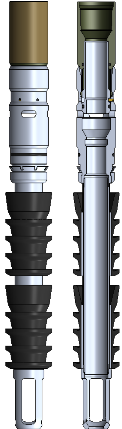
Figure 1 - Typical Torpedo production liner plug assembly.
